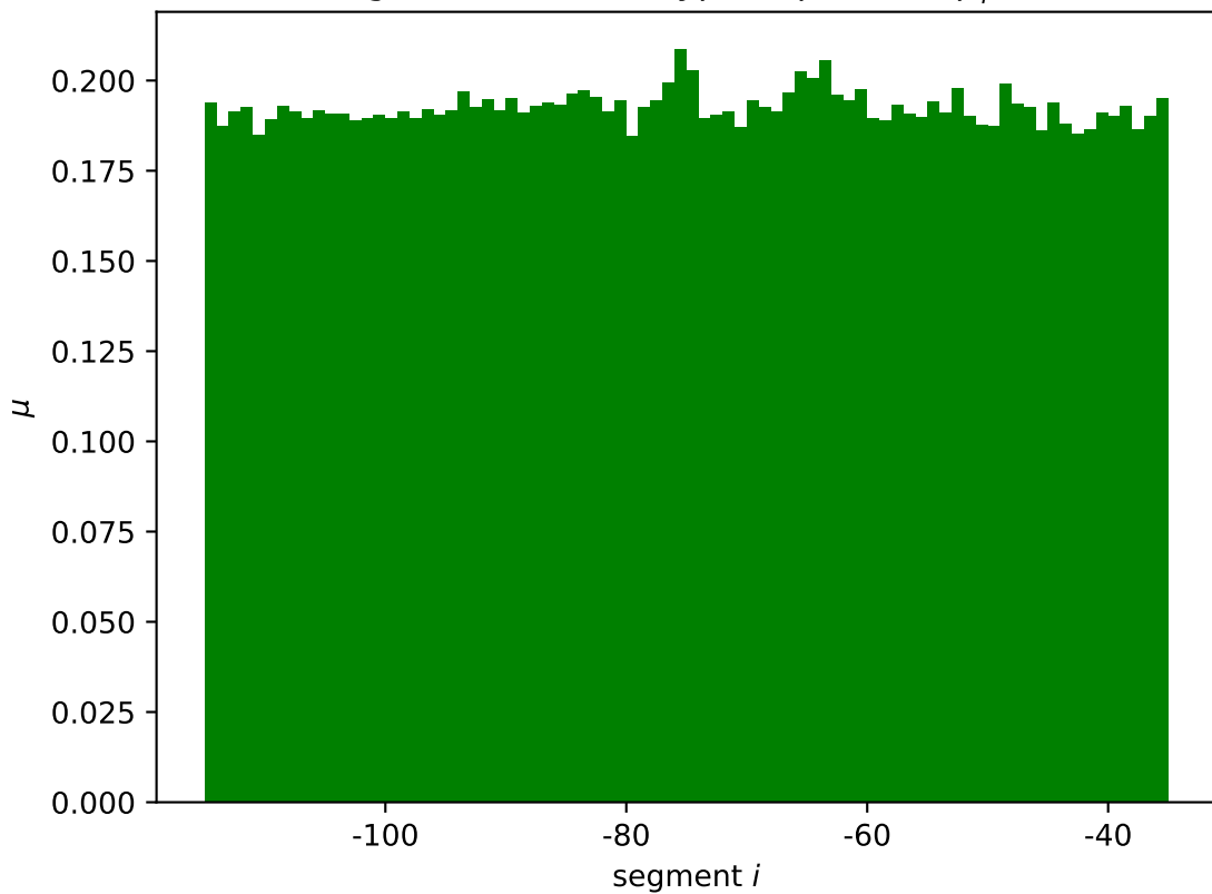
groSL mean wildtype expression \mu_i^*
