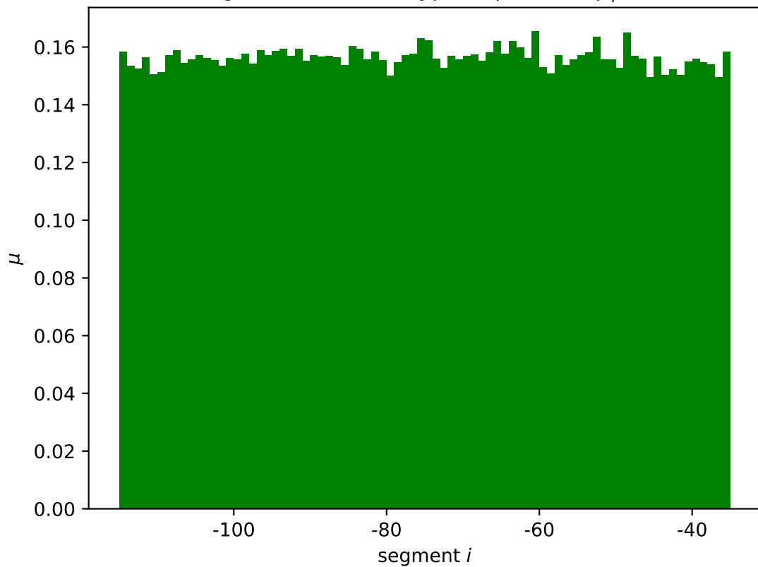
groSL mean wildtype expression \mu_i^*
