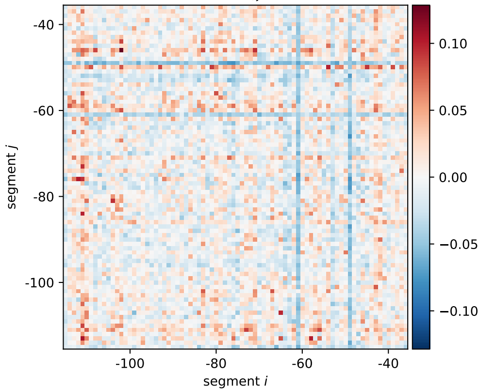
groSL expression shift \xi_{i,j}[0101, 0110, 1010]
