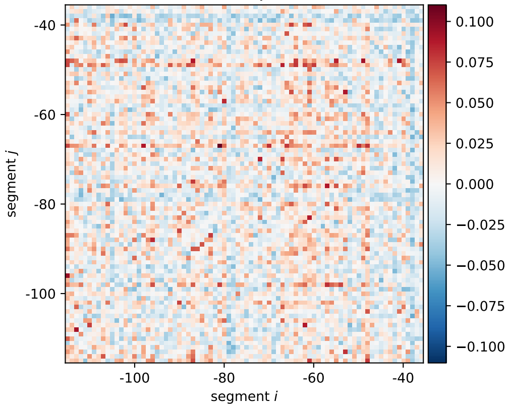
hicB expression shift \xi_{i,j}[0101, 0110, 1010]
