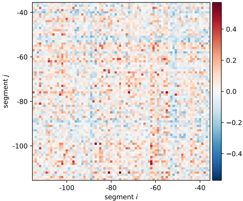
hicB expression shift \xi_{i,j}[0101, 0110, 1010]
