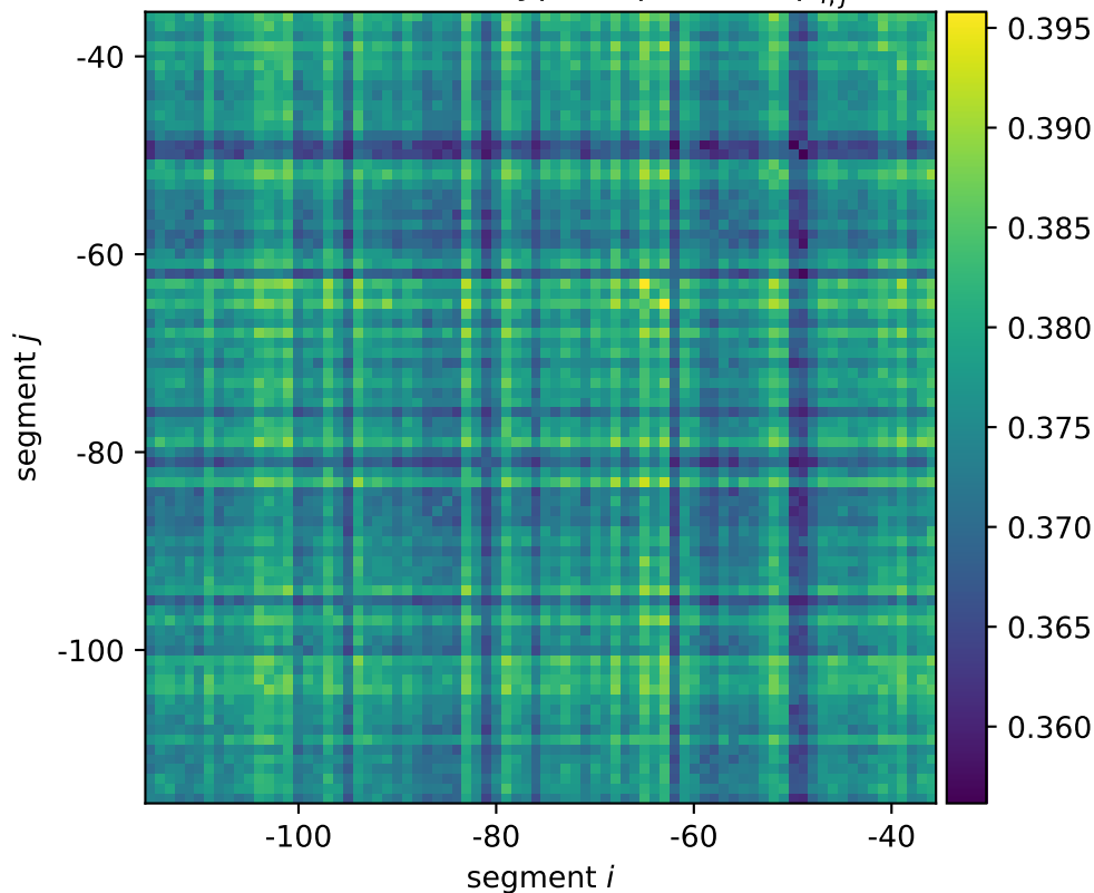
hicB mean wildtype expression \mu_{i,j}^*
