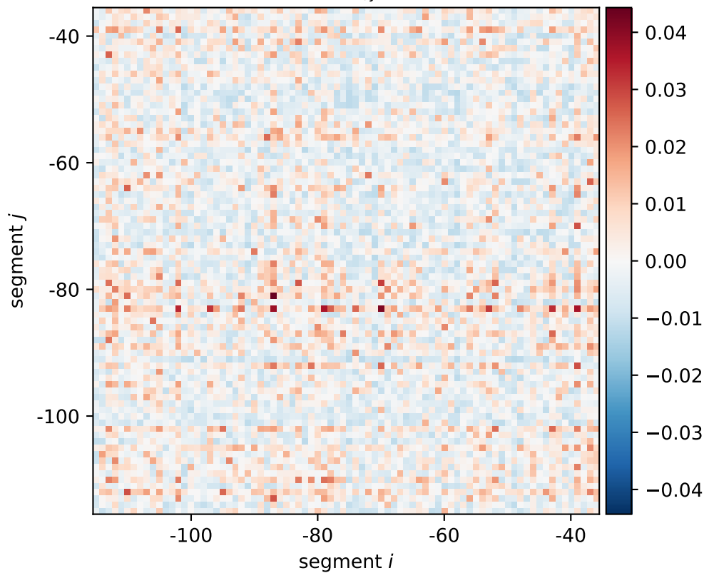
holC expression shift \xi_{i,j}[0101, 0110, 1010]
