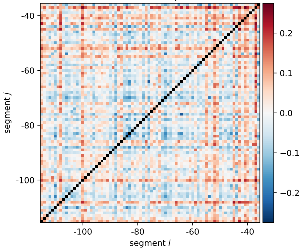
holC expression shift \xi_{i,j}[0011, 1100]
