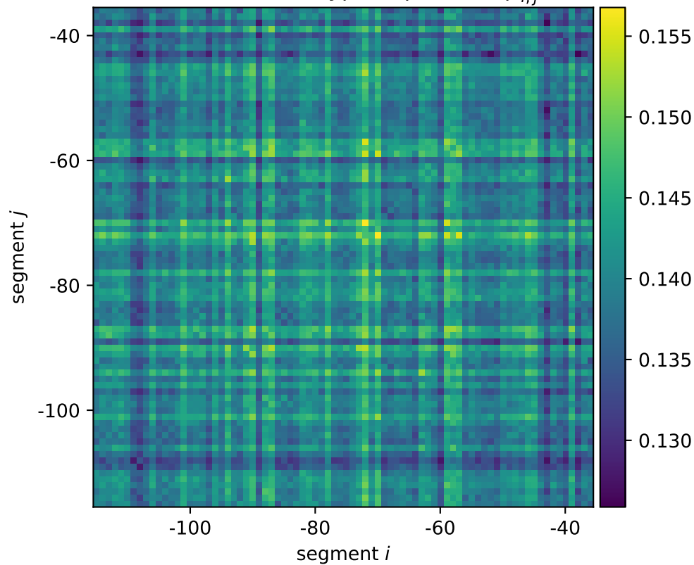
hslU mean wildtype expression \mu_{i,j}^*
