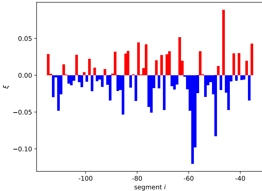
hslU expression shift \xi_i[01, 10]
