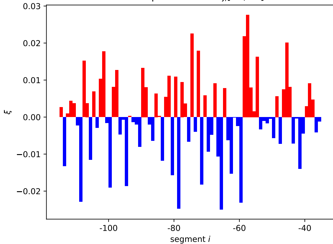
htrB expression shift \xi_i[01, 10]
