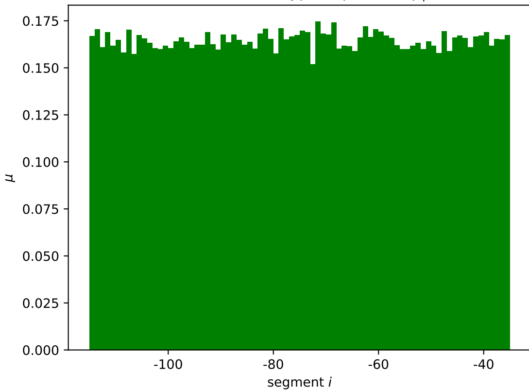
htrB mean wildtype expression \mu_i^*
