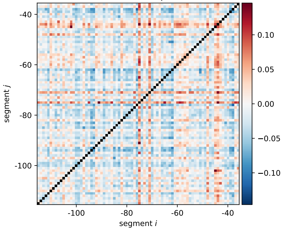
htrB expression shift \xi_{i,j}[0011, 1100]
