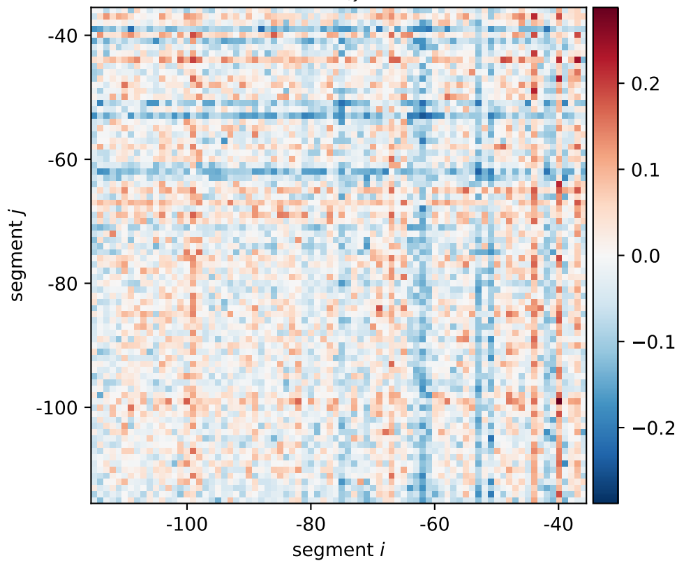
iap expression shift \xi_{i,j}[0101, 0110, 1010]
