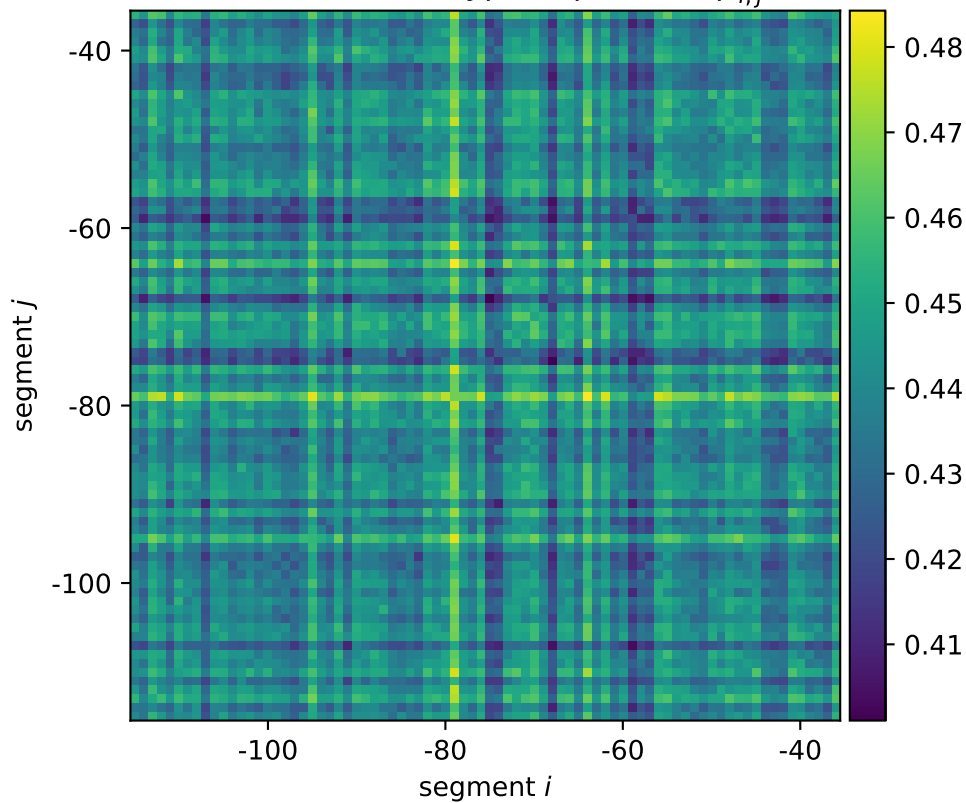
idnK mean wildtype expression \mu_{i,j}^*
