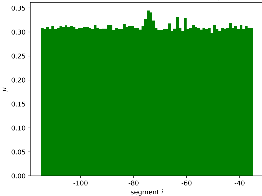
leuABCD mean wildtype expression \mu_i^*
