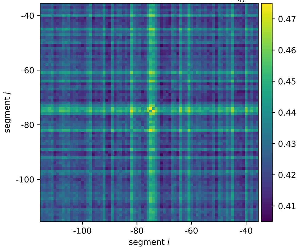
leuABCD mean wildtype expression \mu_{i,j}^*
