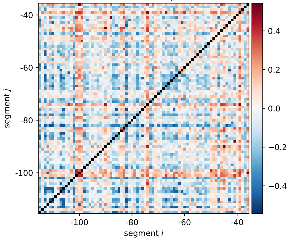
maoP expression shift \xi_{i,j}[\text{0011}, \text{1100}]
