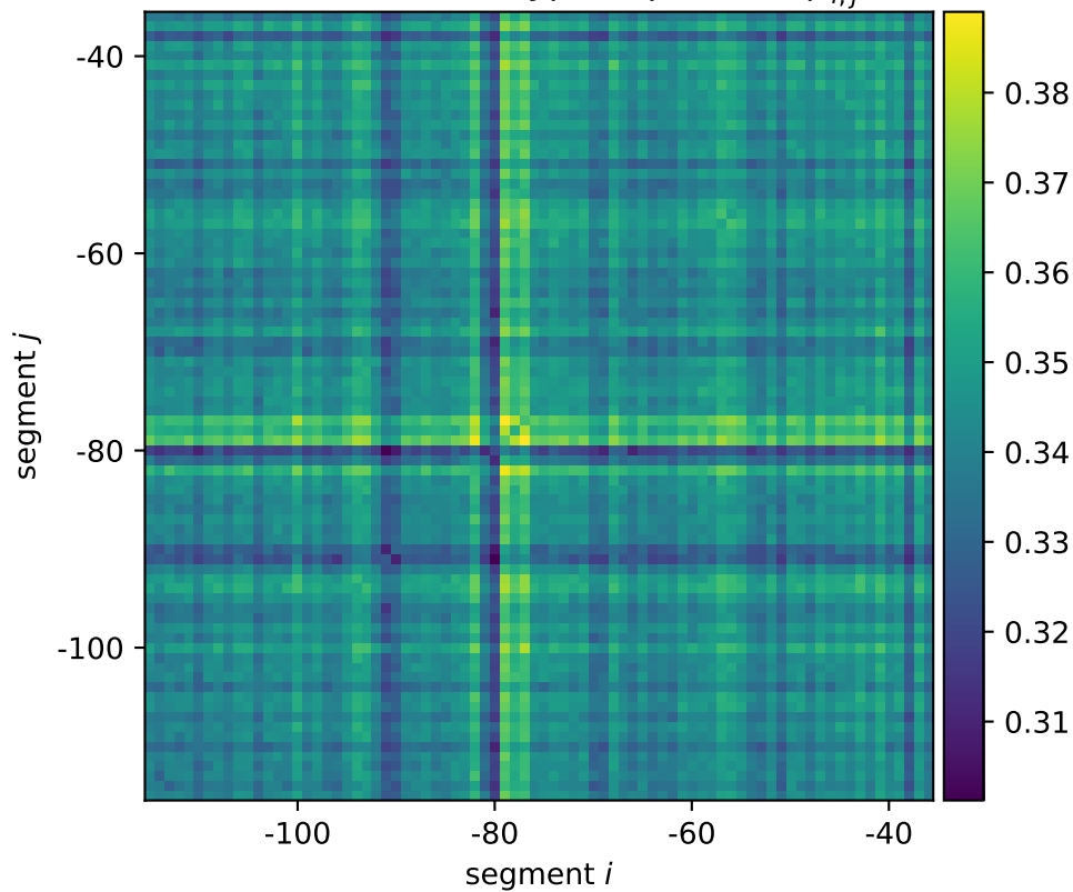
maoP mean wildtype expression \mu_{i,j}^*
