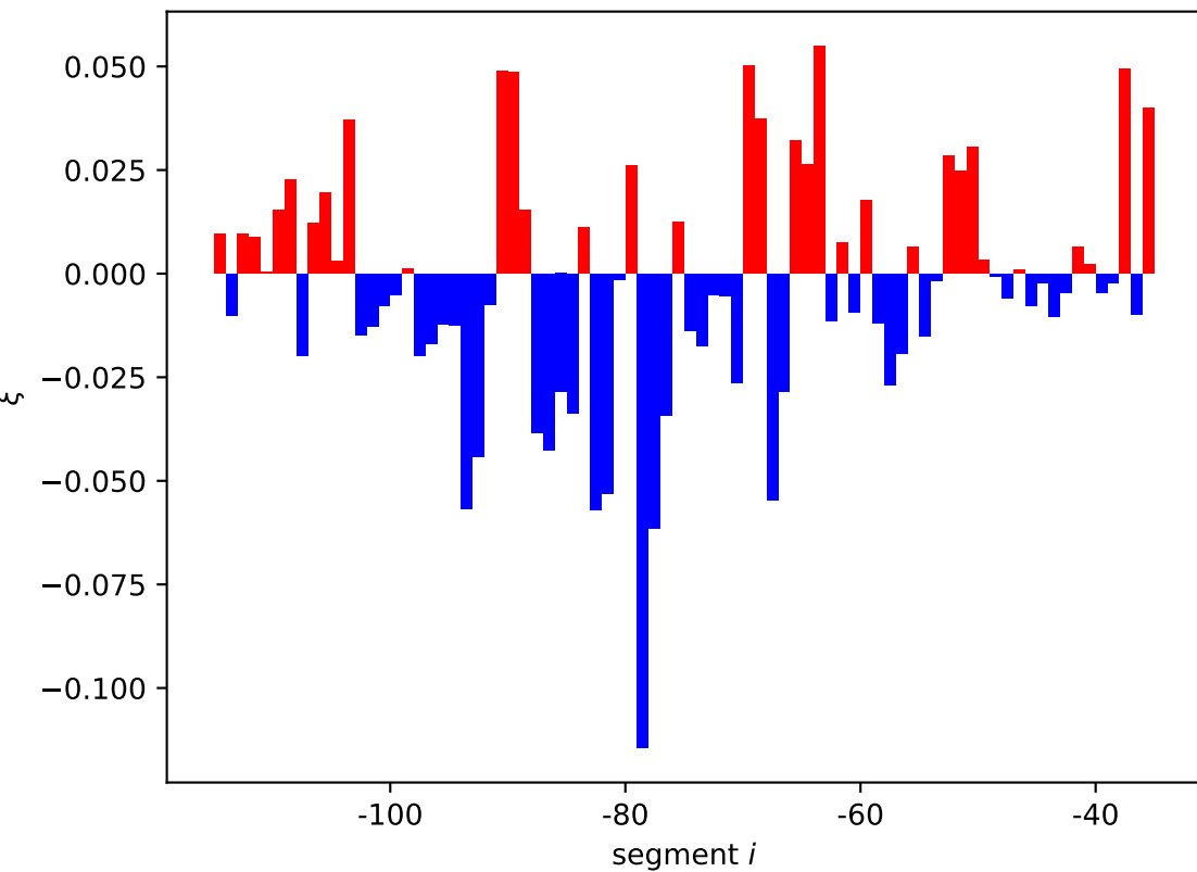
maoP expression shift \xi_i[01, 10]
