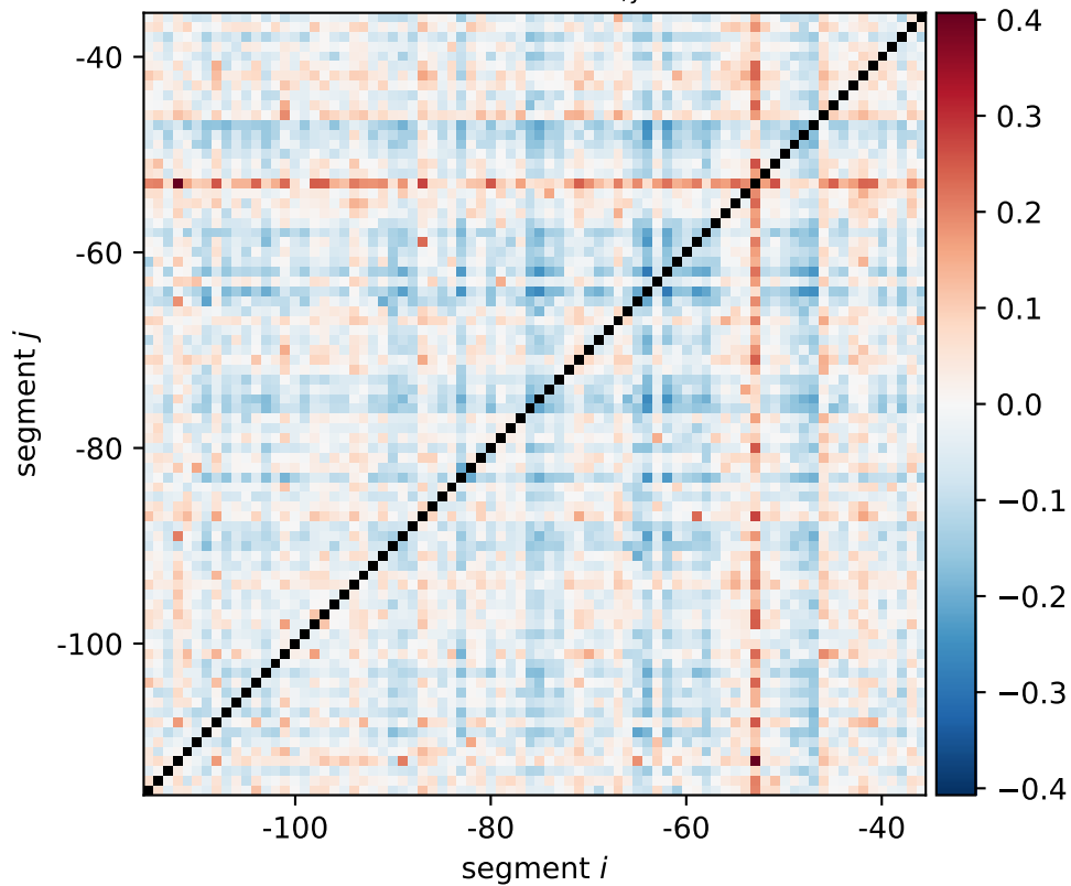
minC expression shift \xi_{i,j}[\text{0011}, \text{1100}]
