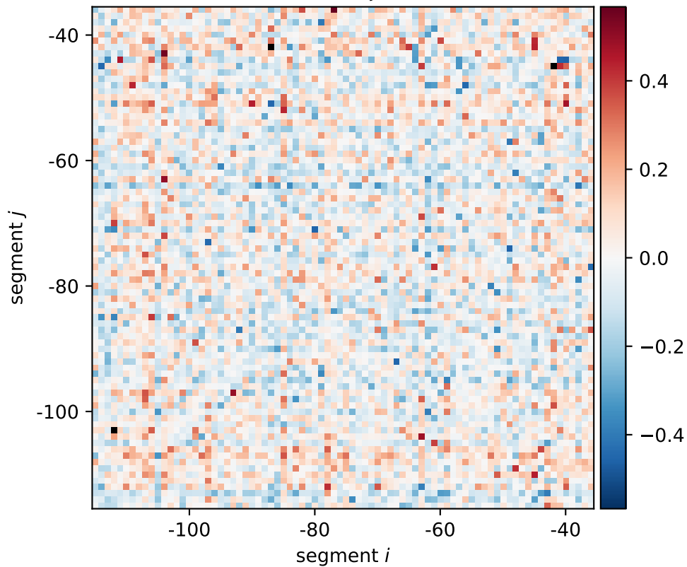
minC expression shift \xi_{i,j}[\text{0101}, \text{0110}, \text{1010}]
