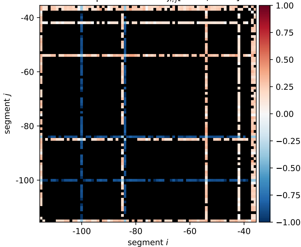
minC expression shift \xi_{i,j}[0011, 1100]
