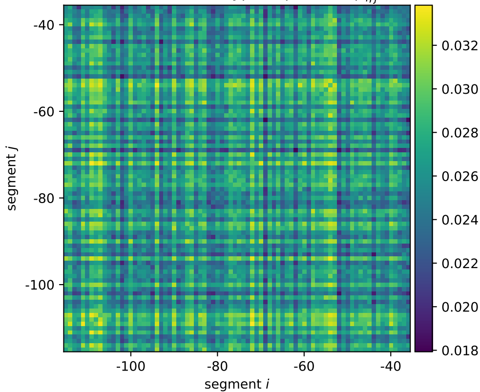
modE mean wildtype expression \mu_{i,j}^*
