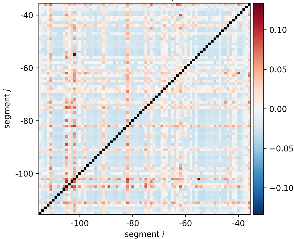
modE expression shift \xi_{i,j}[\text{0011}, \text{1100}]
