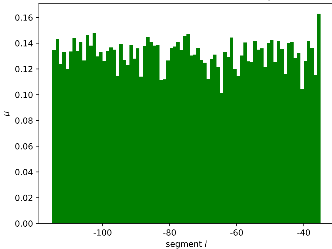
modE mean wildtype expression \mu_i^*
