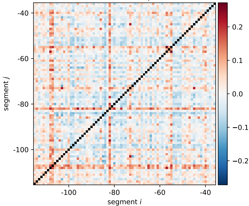
modE expression shift \xi_{i,j}[0011, 1100]
