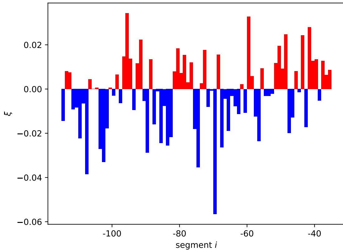
modE expression shift \xi_i[01, 10]
