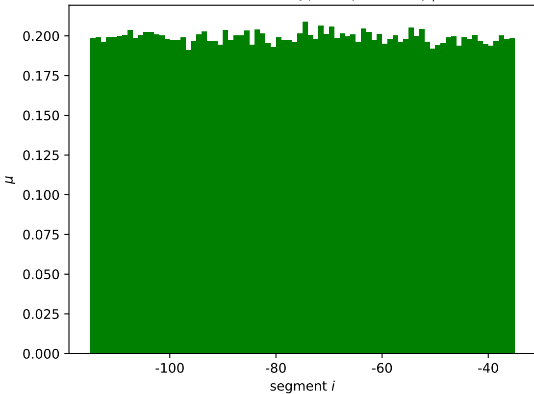
modE mean wildtype expression \mu_i^*
