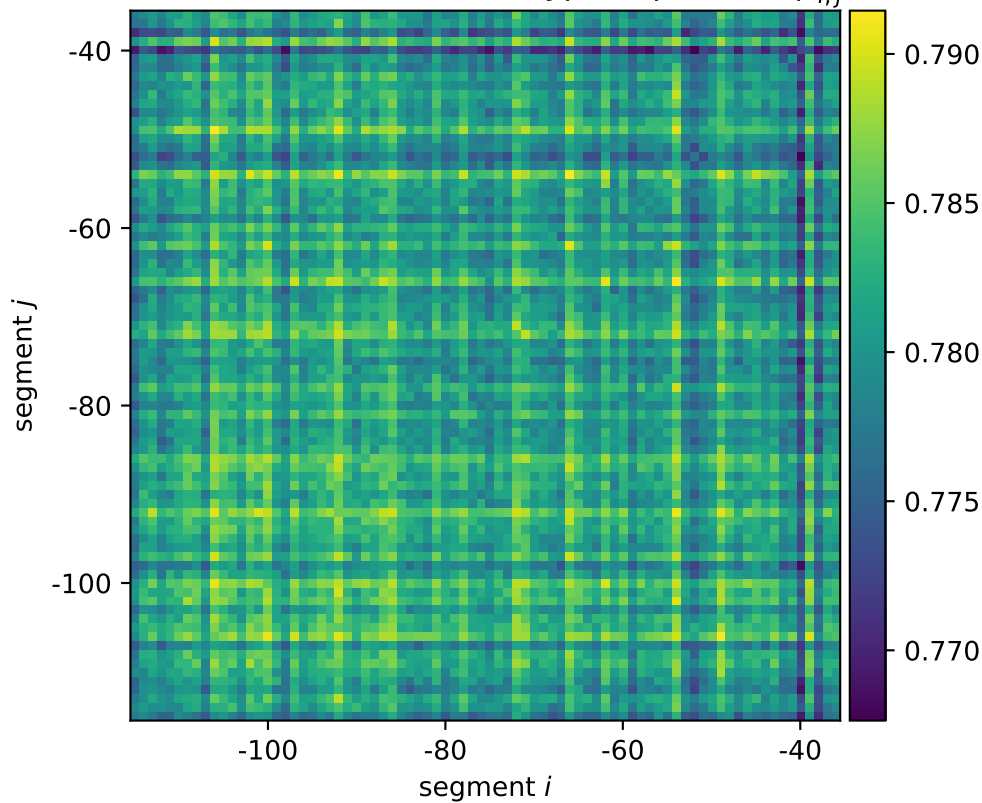
motAB-cheAW mean wildtype expression \mu_{i,j}^*
