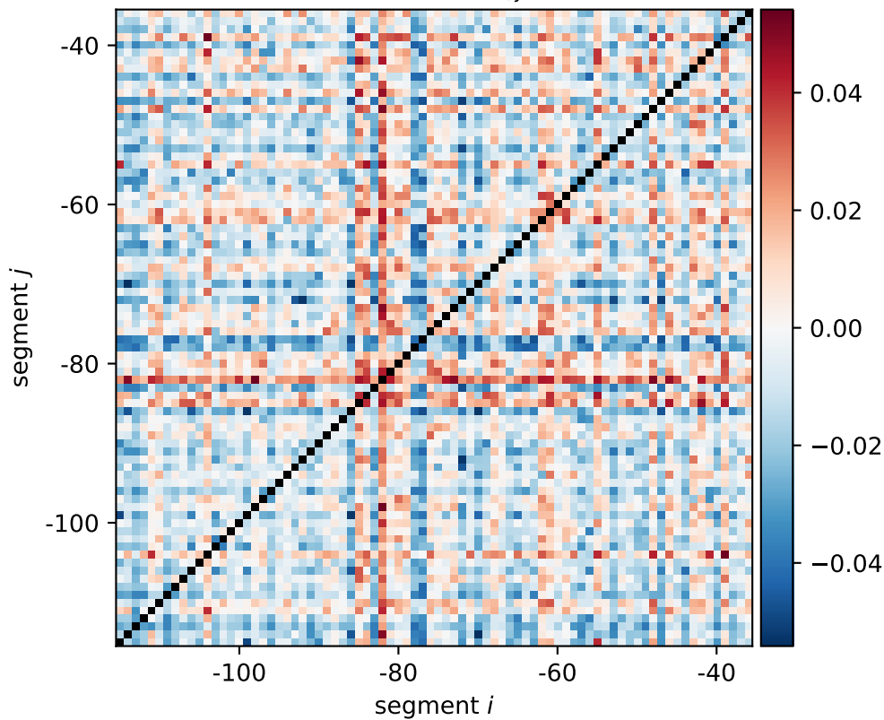
mscK expression shift \xi_{i,j}[\text{0011}, \text{1100}]
