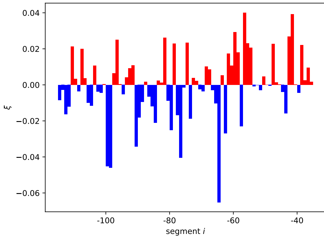
mscK expression shift \xi_i[01, 10]
