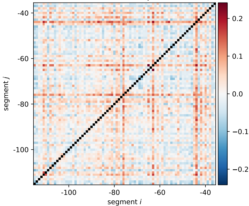
mscK expression shift \xi_{i,j}[0011, 1100]
