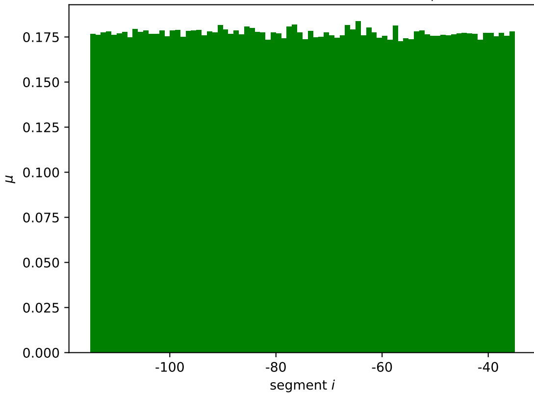
mscK mean wildtype expression \mu_i^*
