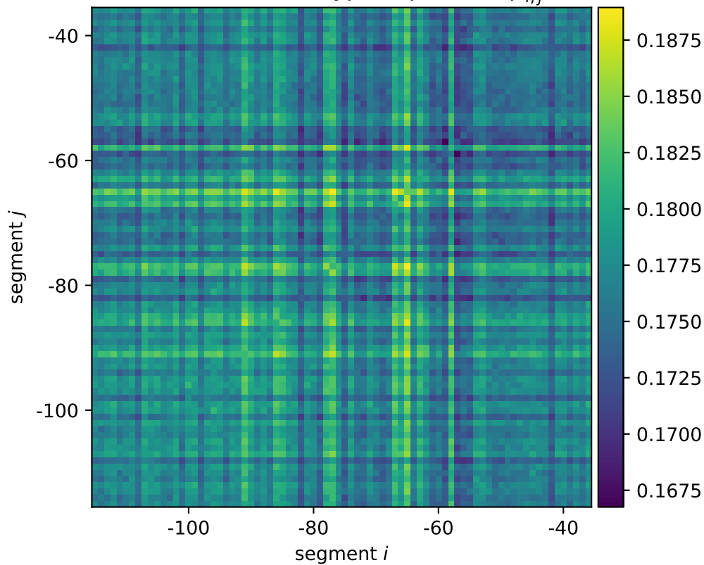
mscK mean wildtype expression \mu_{i,j}^*
