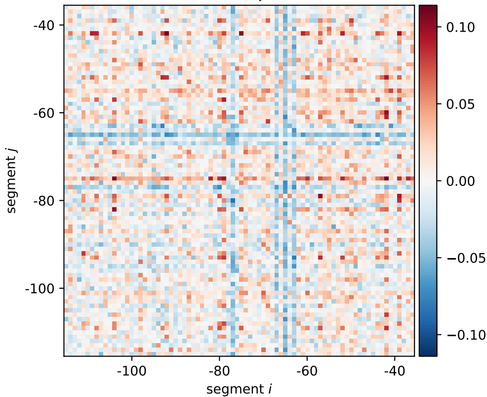
msck expression shift \xi_{i,j}[0101, 0110, 1010]
