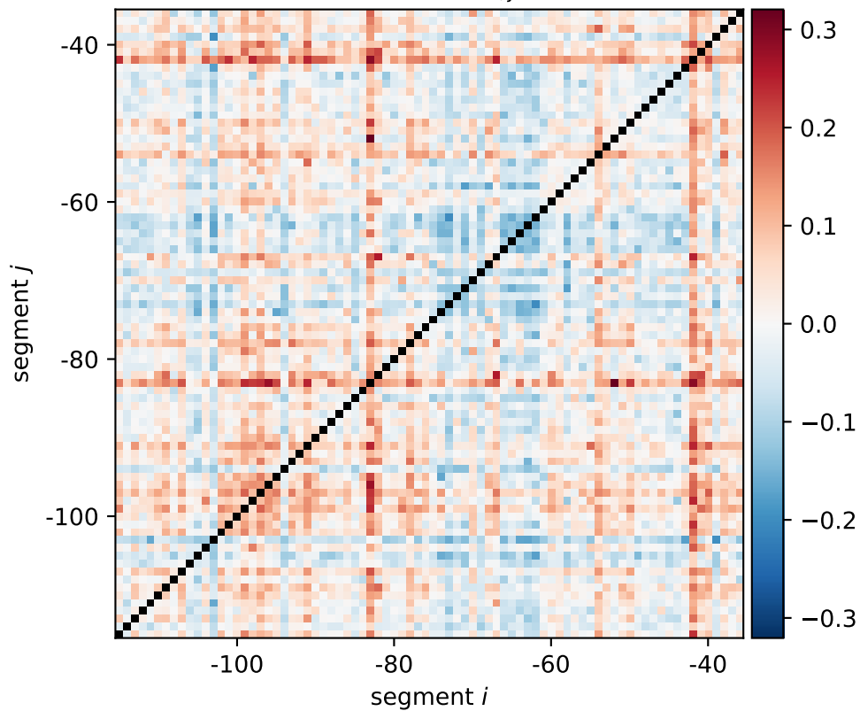
mscL expression shift \xi_{i,j}[\text{0011}, \text{1100}]
