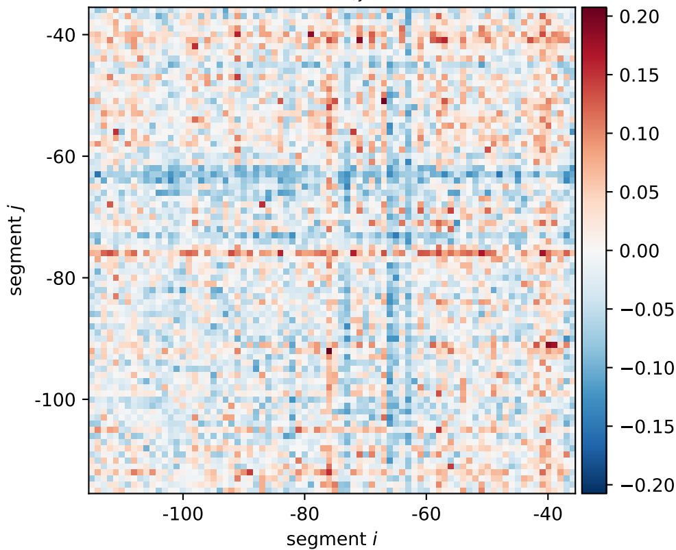
mscL expression shift \xi_{i,j}[0101, 0110, 1010]
