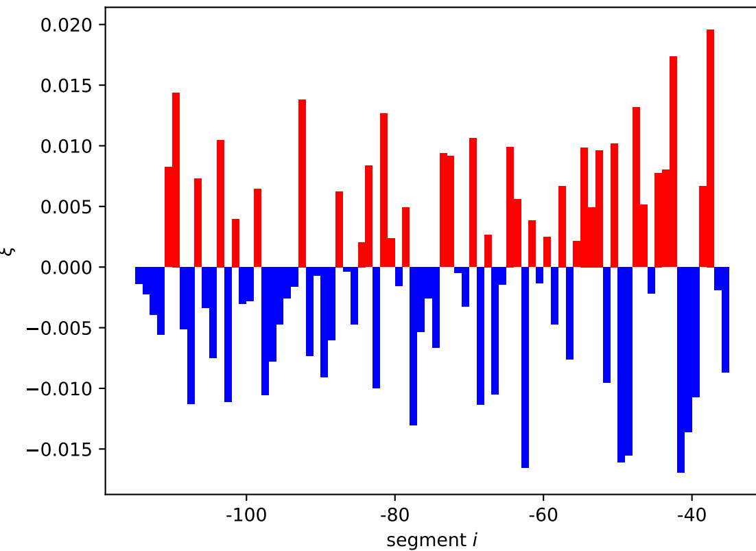
mscM expression shift \xi_i[01, 10]
