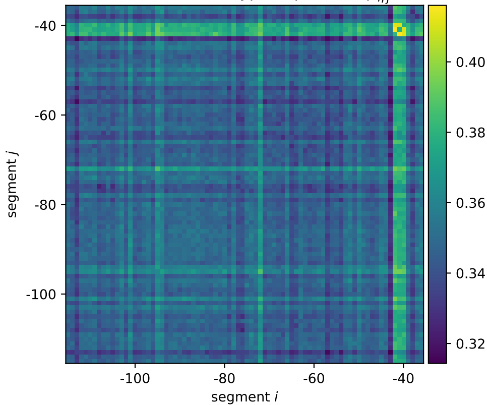
mscM mean wildtype expression \mu_{i,j}^*
