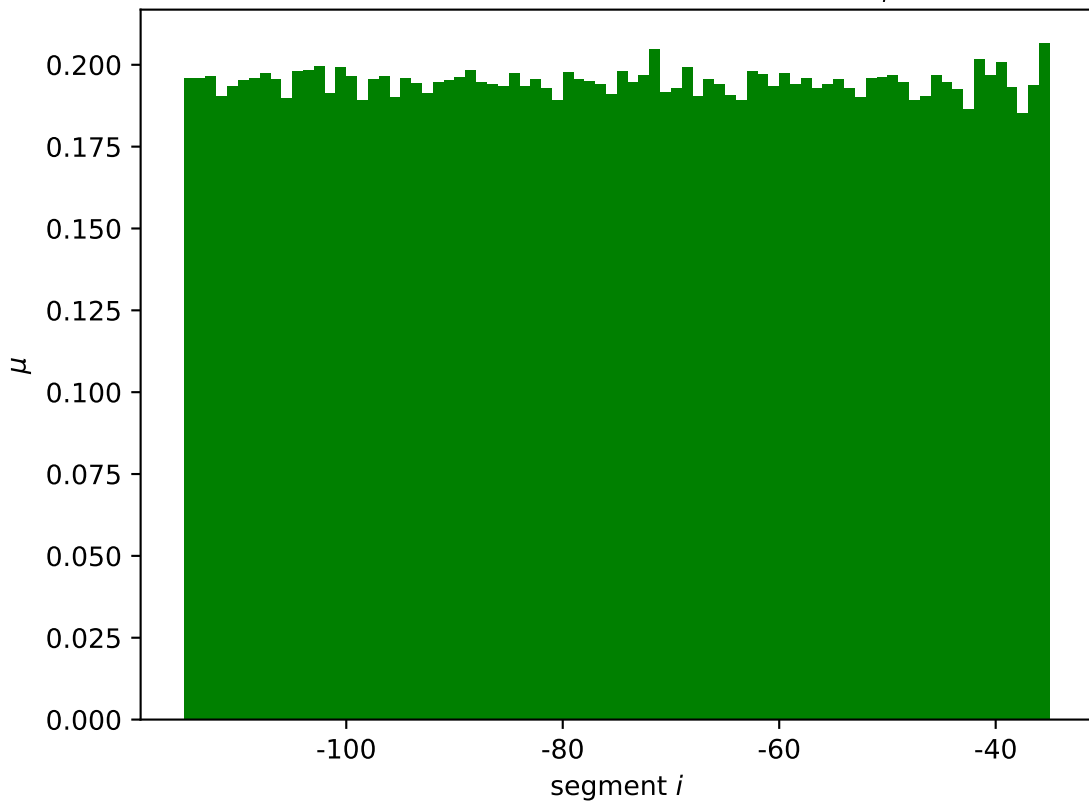
mscM mean wildtype expression \mu_i^*
