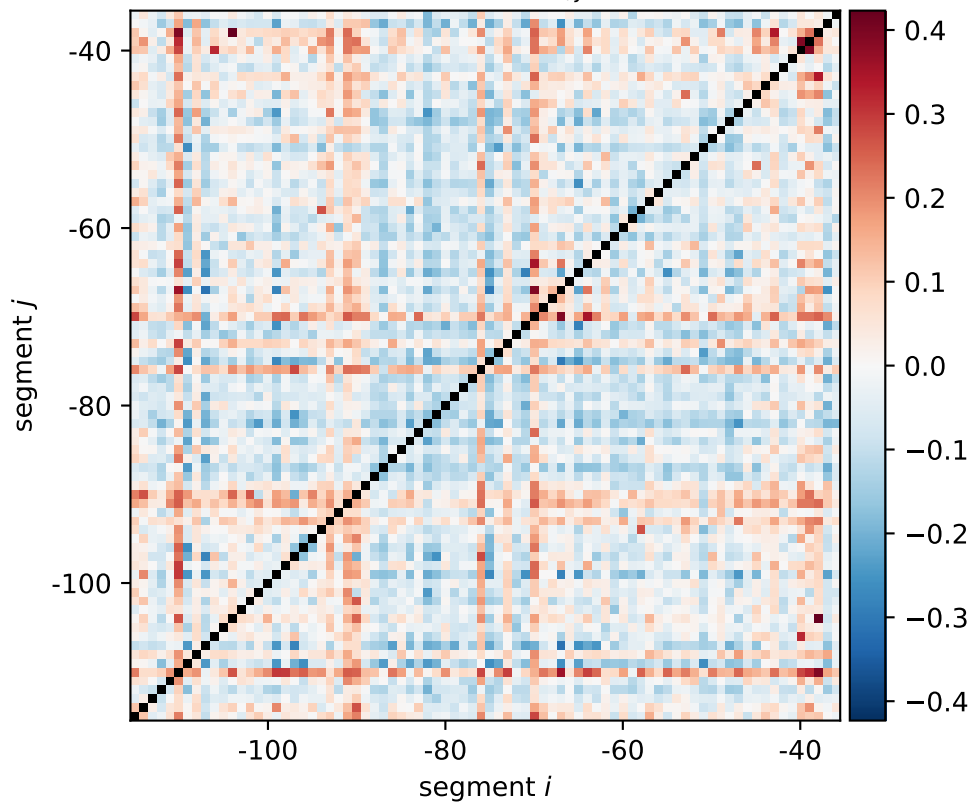
mscS expression shift \xi_{i,j}[\text{0011}, \text{1100}]
