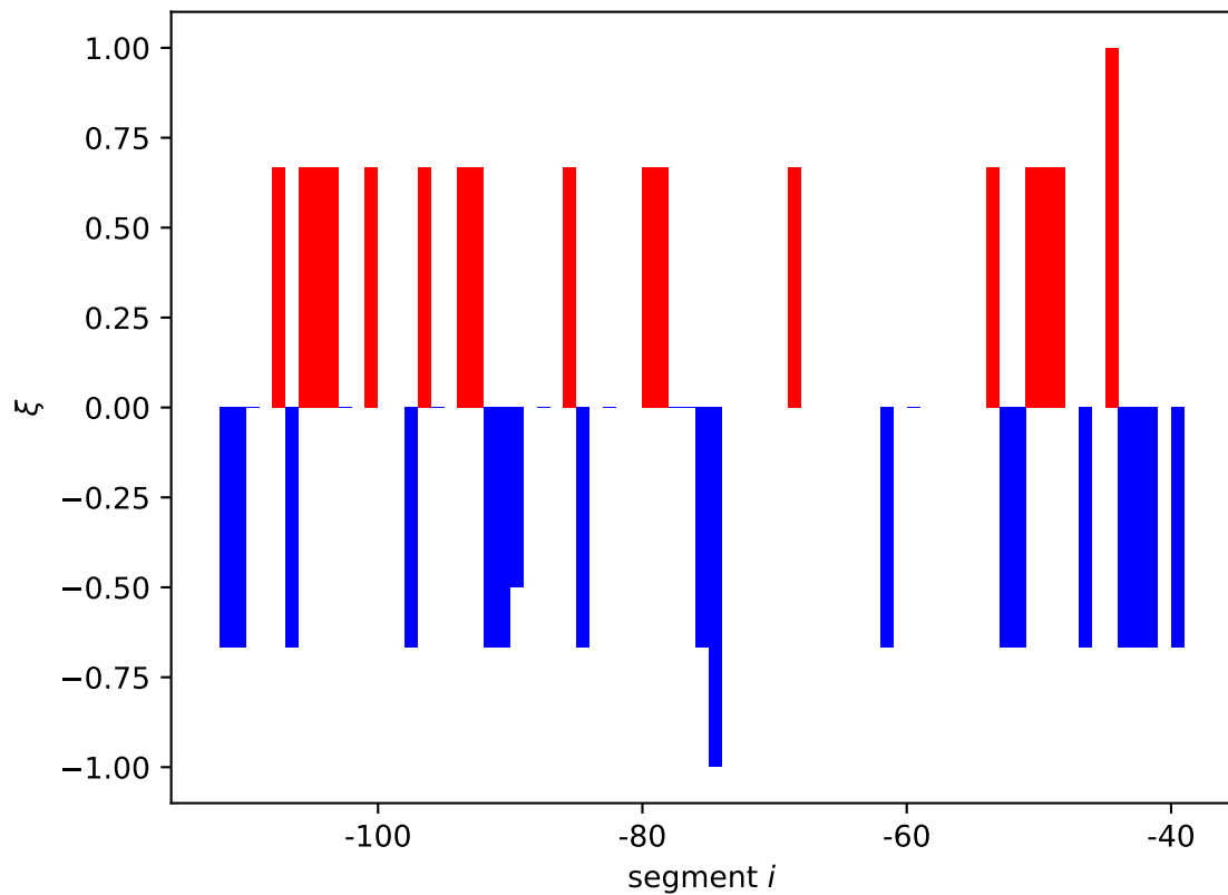
mscS expression shift \xi_i[01, 10]
