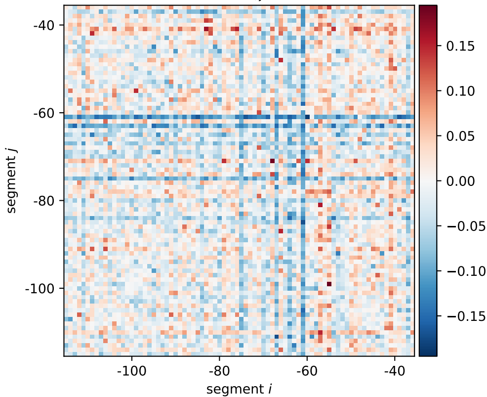
mscS expression shift \xi_{i,j}[0101, 0110, 1010]
