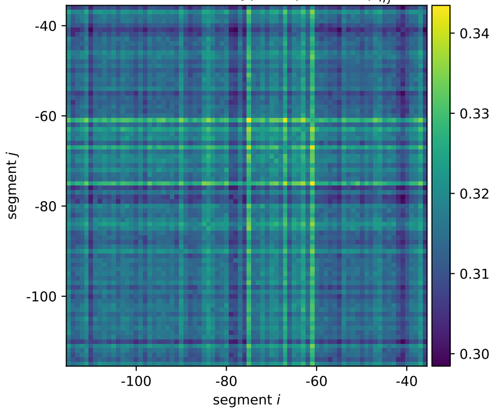
mscS mean wildtype expression \mu_{i,j}^*
