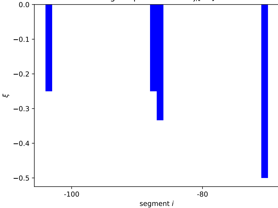
mtgA expression shift \xi_i[11]
