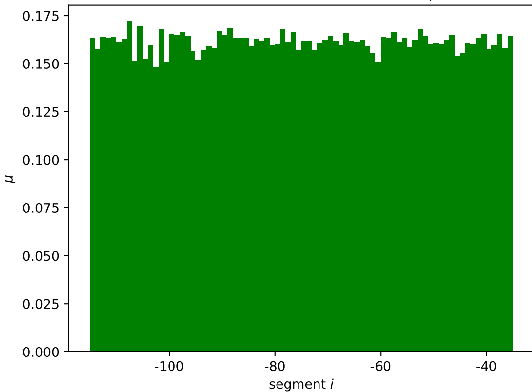
mtgA mean wildtype expression \mu_i^*
