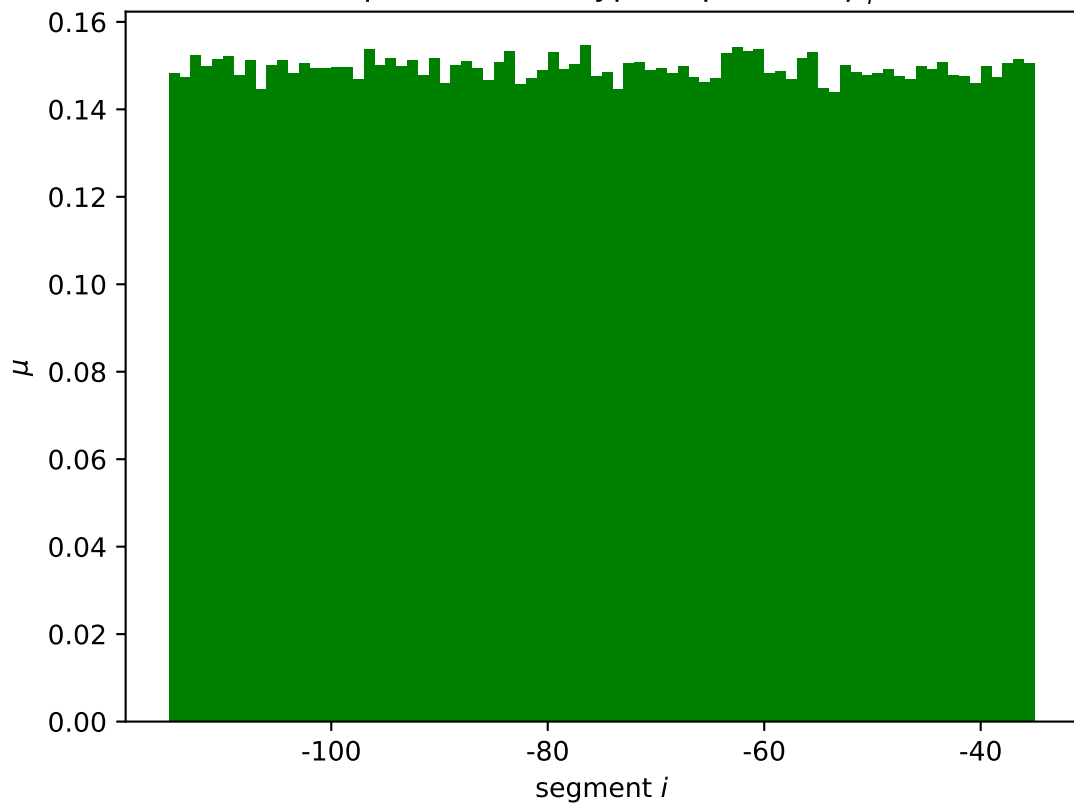
ompR mean wildtype expression \mu_i^*
