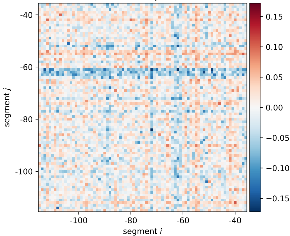
ompR expression shift \xi_{i,j}[0101, 0110, 1010]
