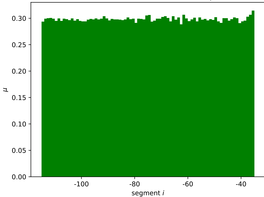
pcm mean wildtype expression \mu_i^*
